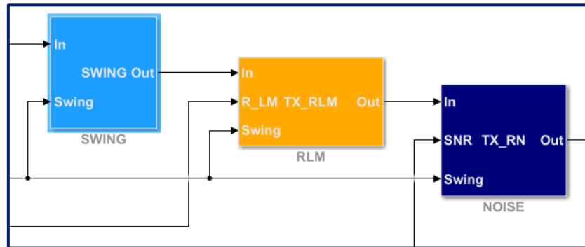
TX IBIS-AMI model block diagram
