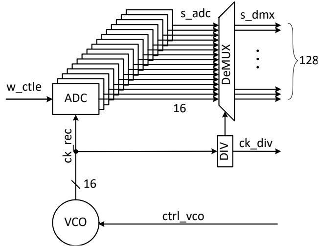
16-way time-interleaved ADC 128-sample DSP frame
